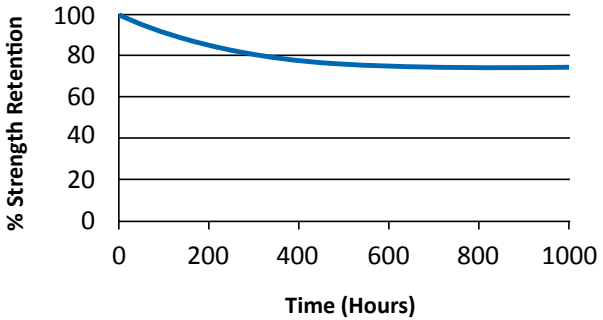
Thermal Ageing at 180°C (356°F)
