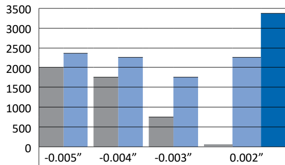
Retaining Compounds vs. Press Fits
