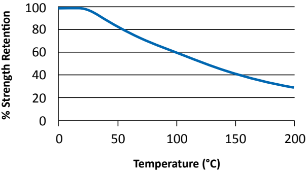
Hot Strength
