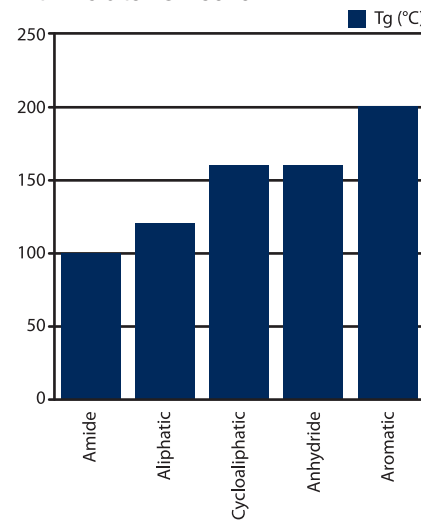
Hardener Tg Overview with Araldite® GY 6010
