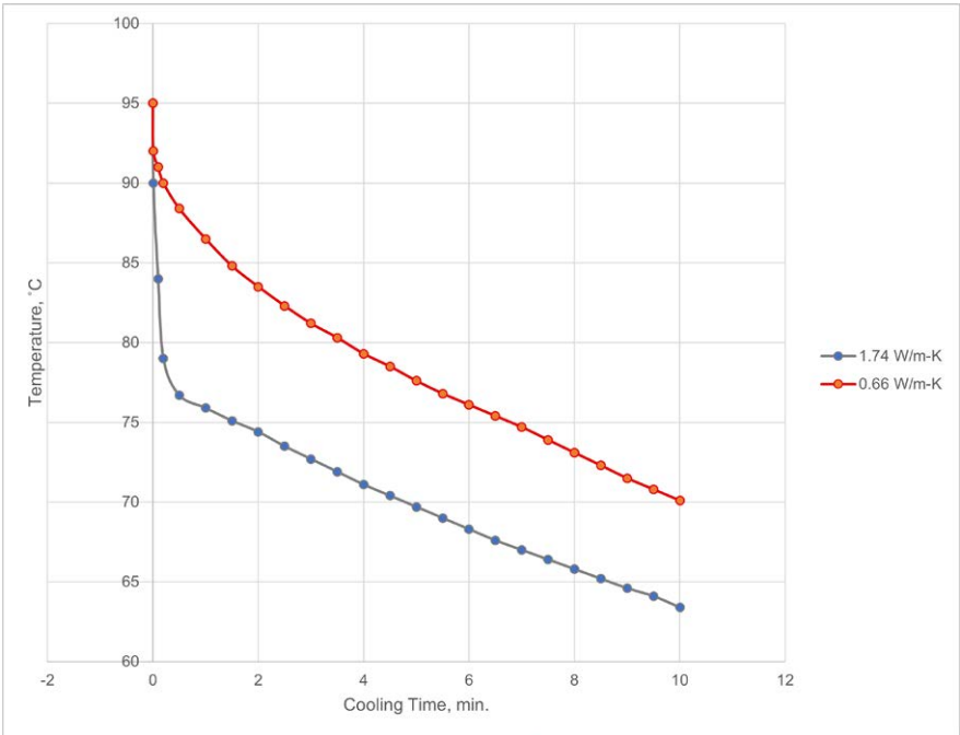
Thermal Conductivity Graph
