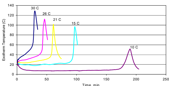
Typical Exotherm Curve for MA550 in a 30 gm Mass at Various Ambient Temperatures 5
